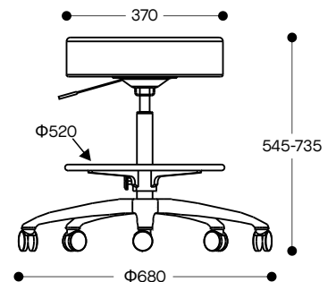
Stool with 5-star base and optional foot ring
