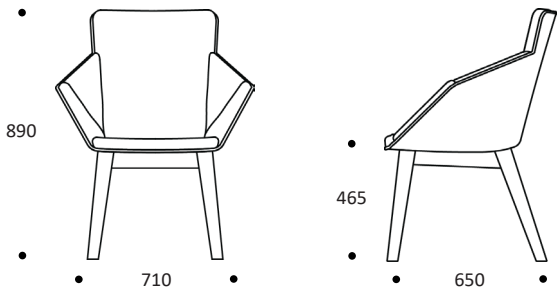
Timber Base
